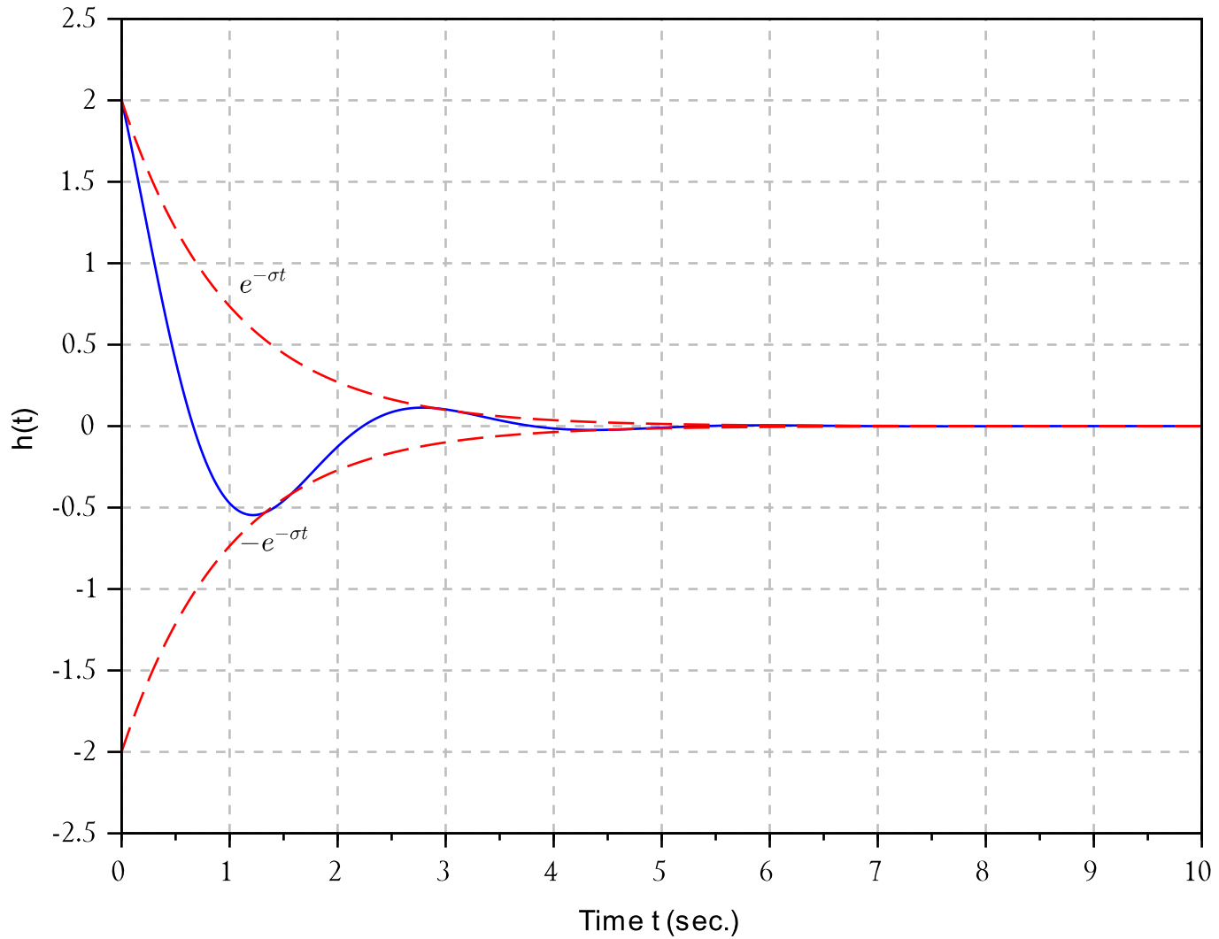
Impulse response of the underdamped system
