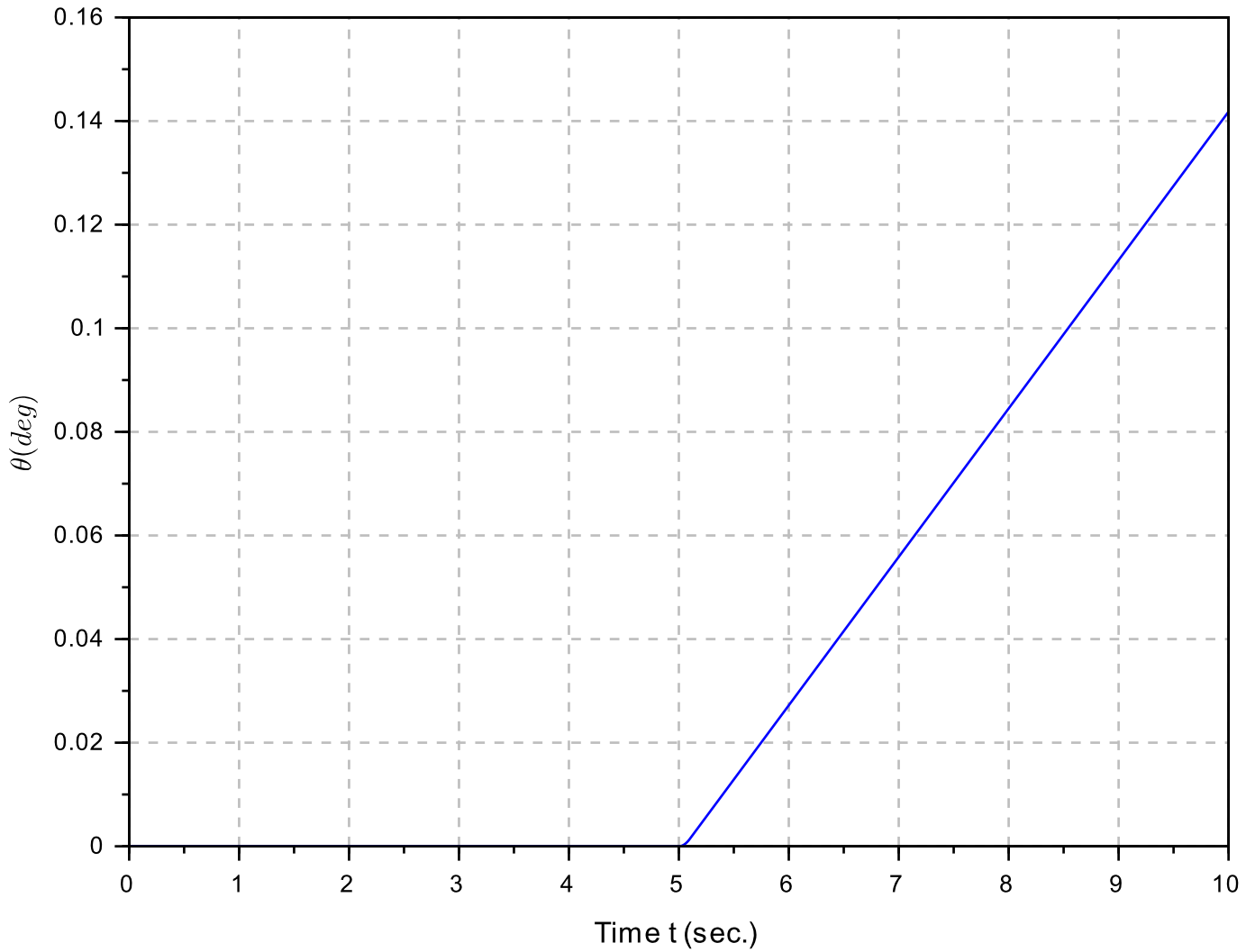
Transient response of the satellite(double-pulse) (b) satellite attitude
