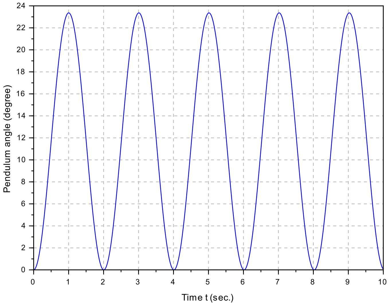
Response of pendulum to a step input in the applied torque
