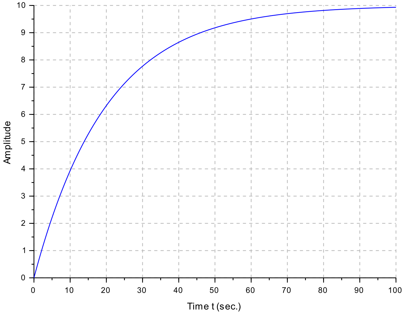
Responses of car velocity to a step in u
