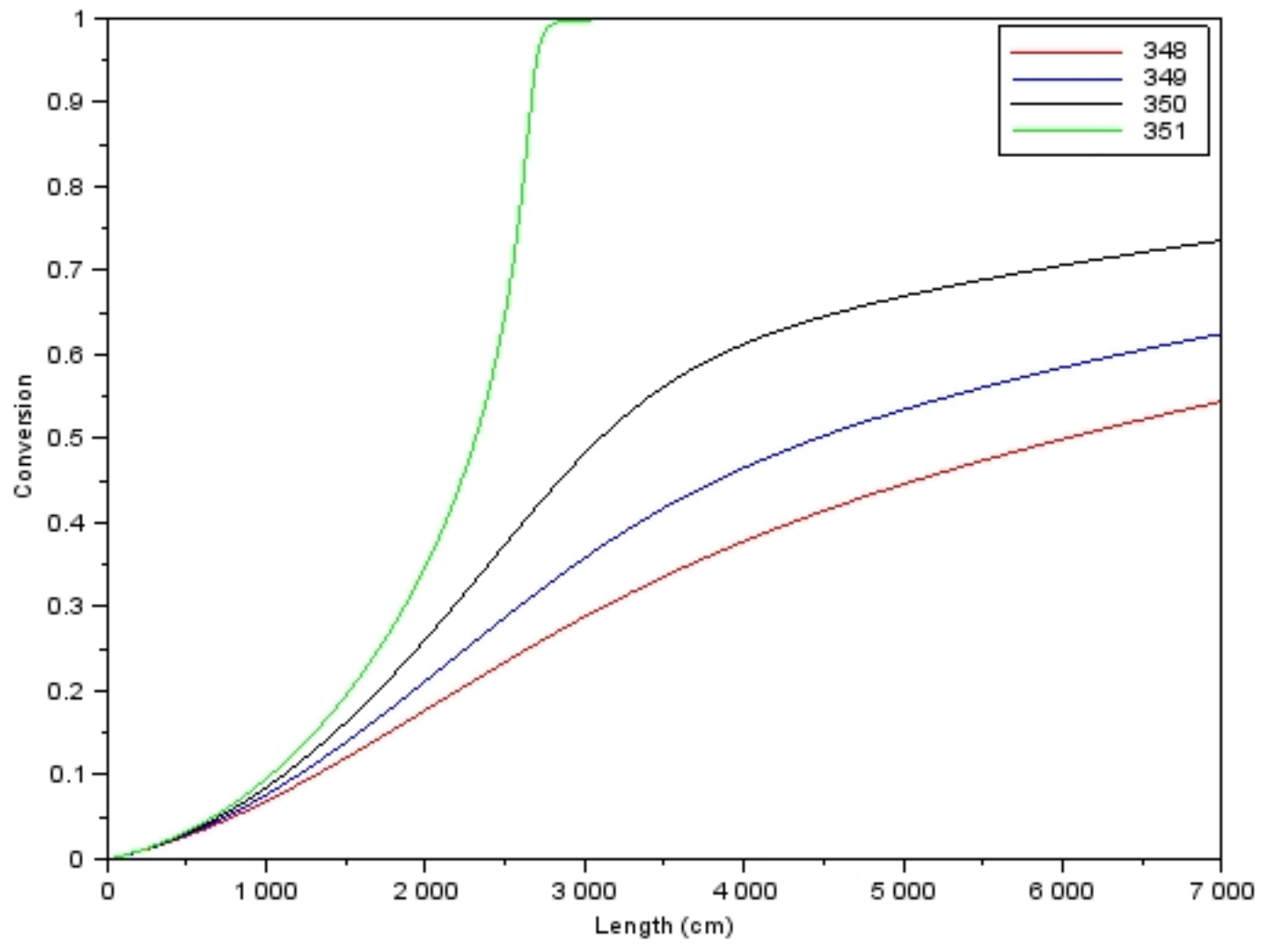
Conversion for a jacketed tubular reactor
