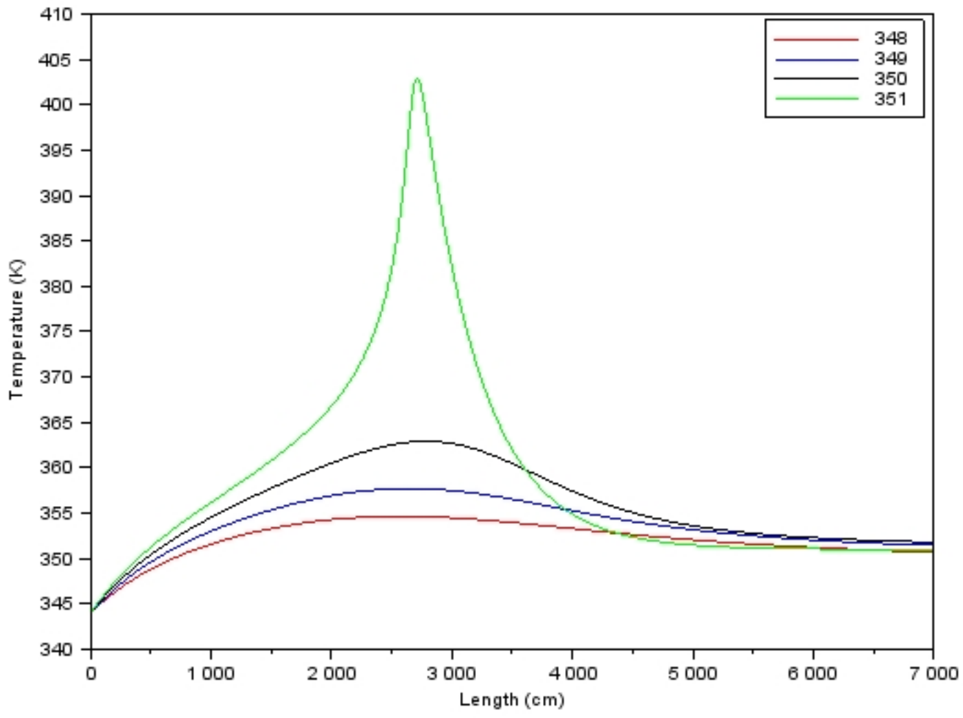
Temperature Profiles for a jacketed tubular reactor
