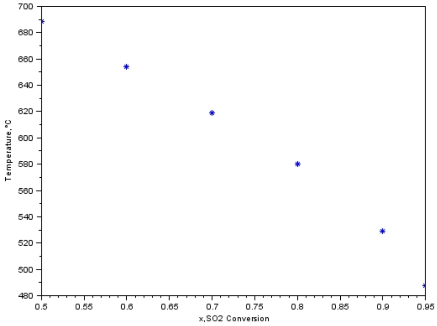
Temperature in Stage 1 of an SO 2 converter
