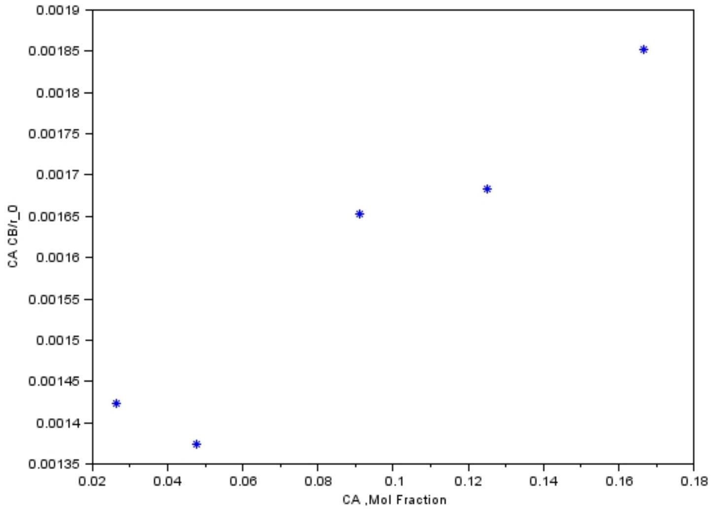
Test of Eley-Rideal model for benzene alkylation
